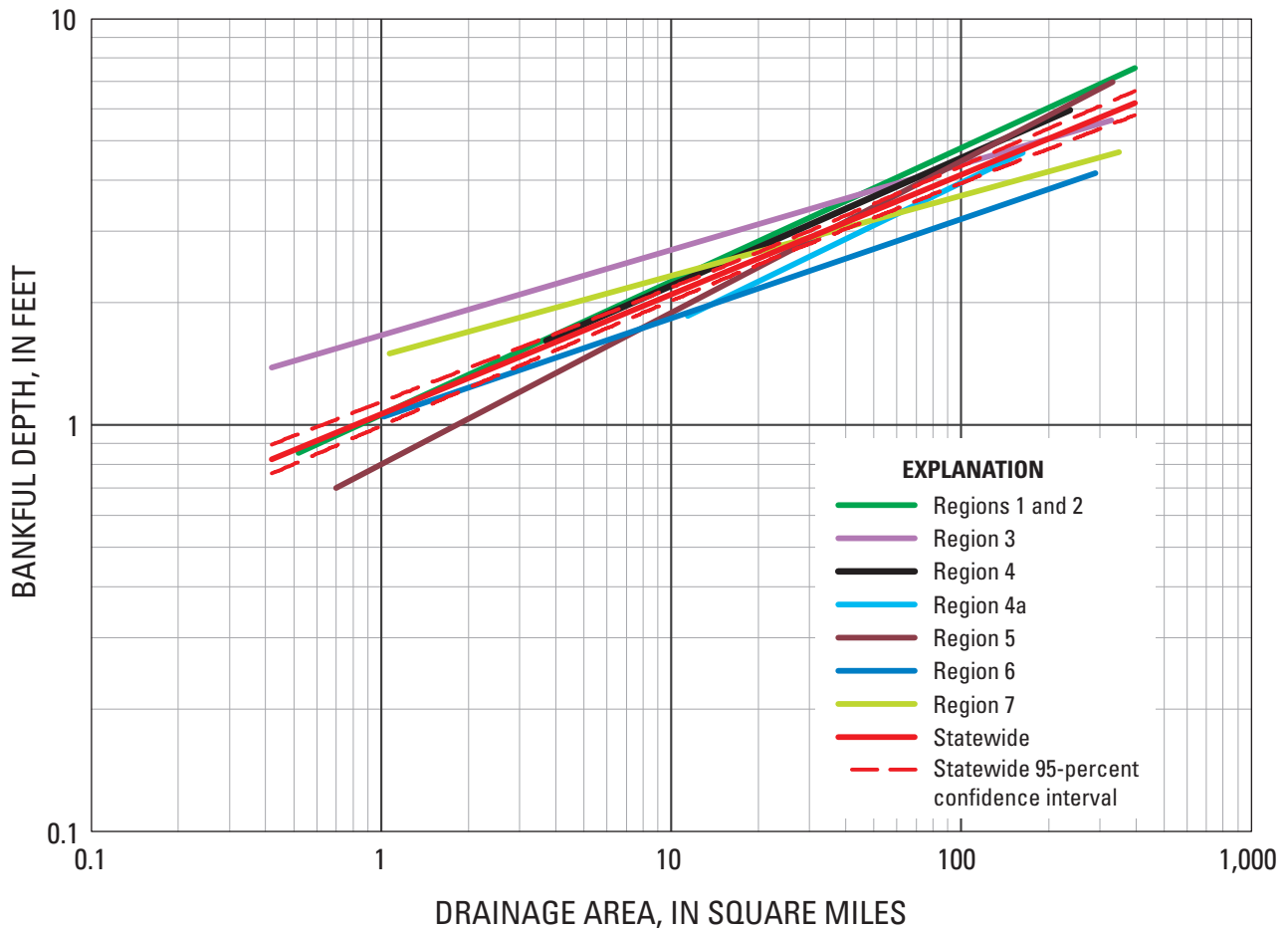
Figure 5. Bankfull depth as a function of drainage area for seven hydrologic regions in New York State and statewide.
