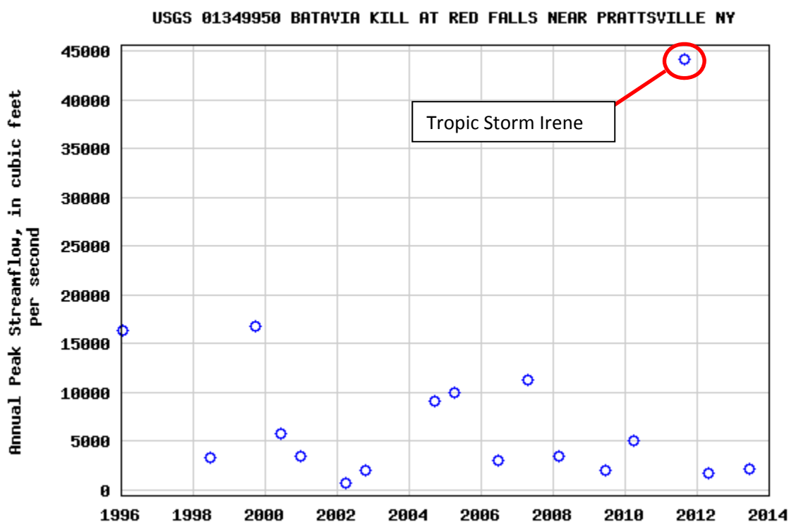
Figure 3-1: Annual Peak Discharge - USGS Gauge #01349950 at Red Falls, at STA 98+00
