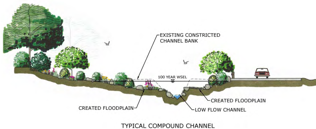
Figure 4-4: Typical Cross Section of a Compound Channel
