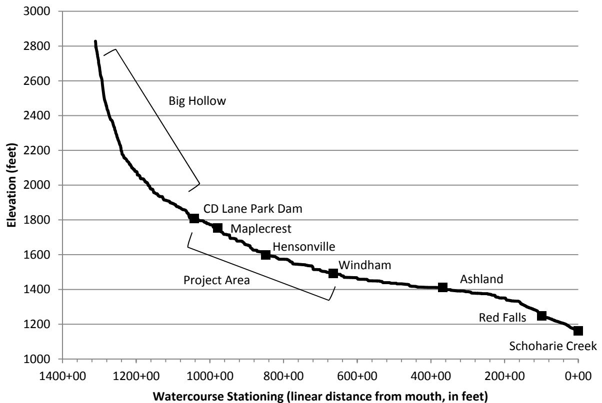
Figure 2-2: Batavia Kill Channel Profile
