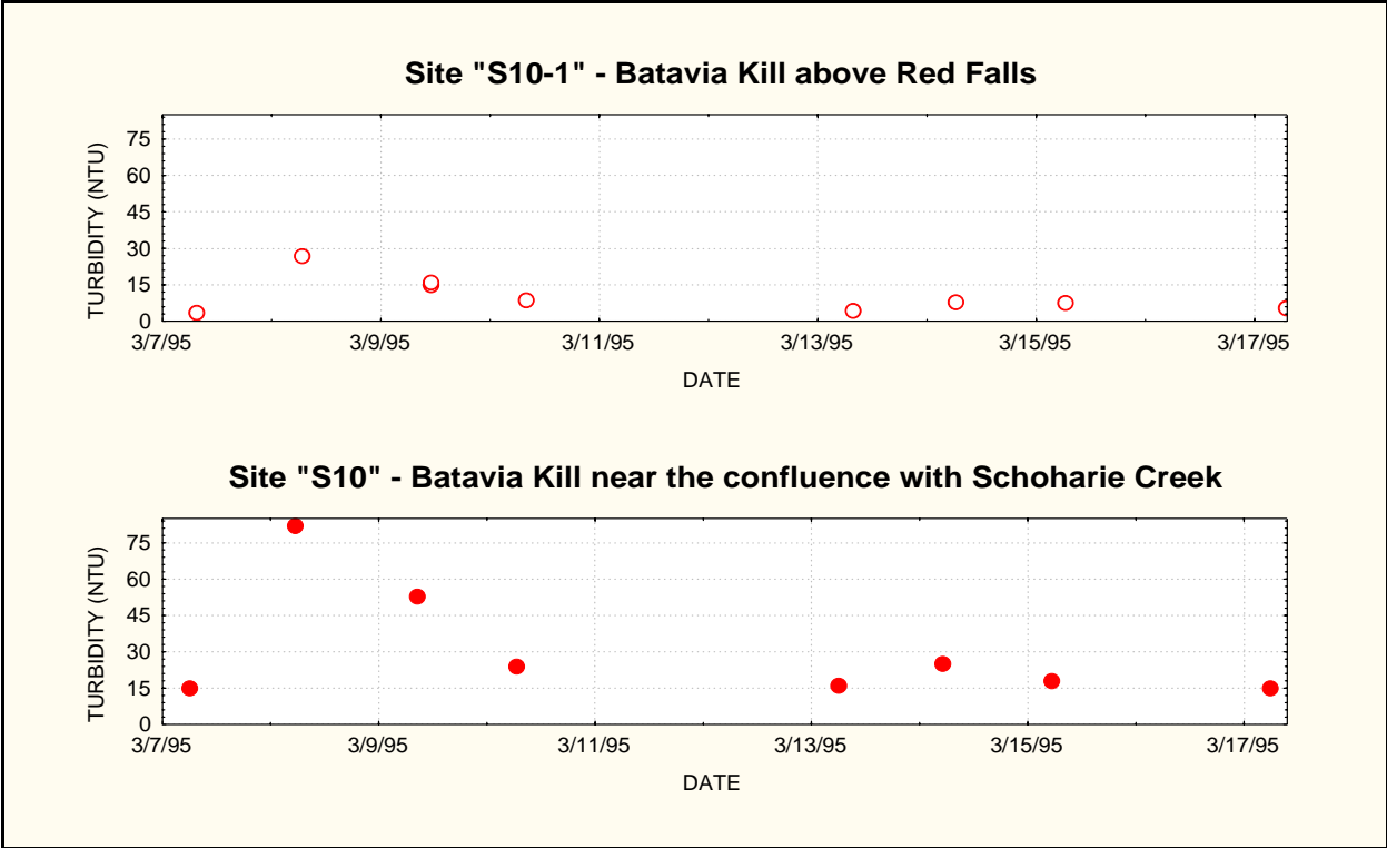
Figure V-5: Turbidity above and below Red Falls, March 1995.
