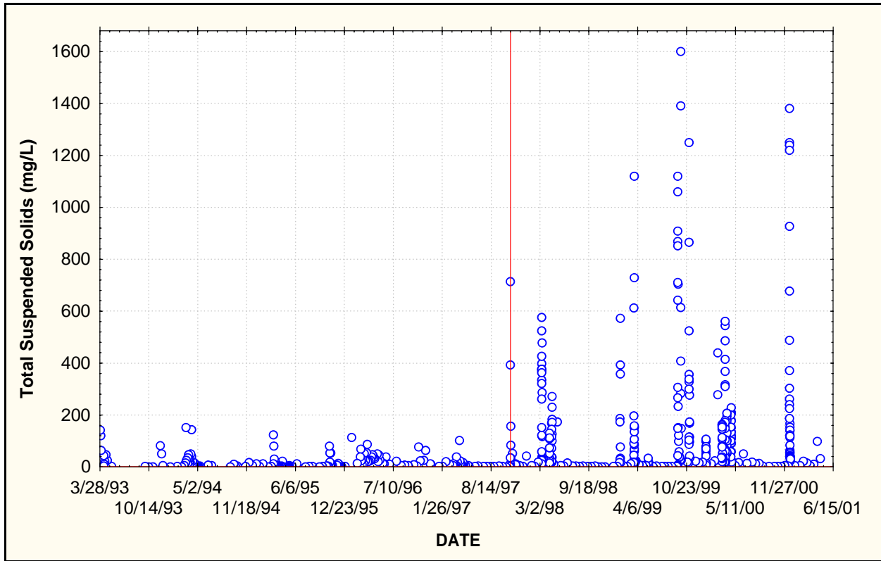
Figure V-3: Historical Total Suspended Solids (TSS) data for site S-10 on the Batavia Kill.
