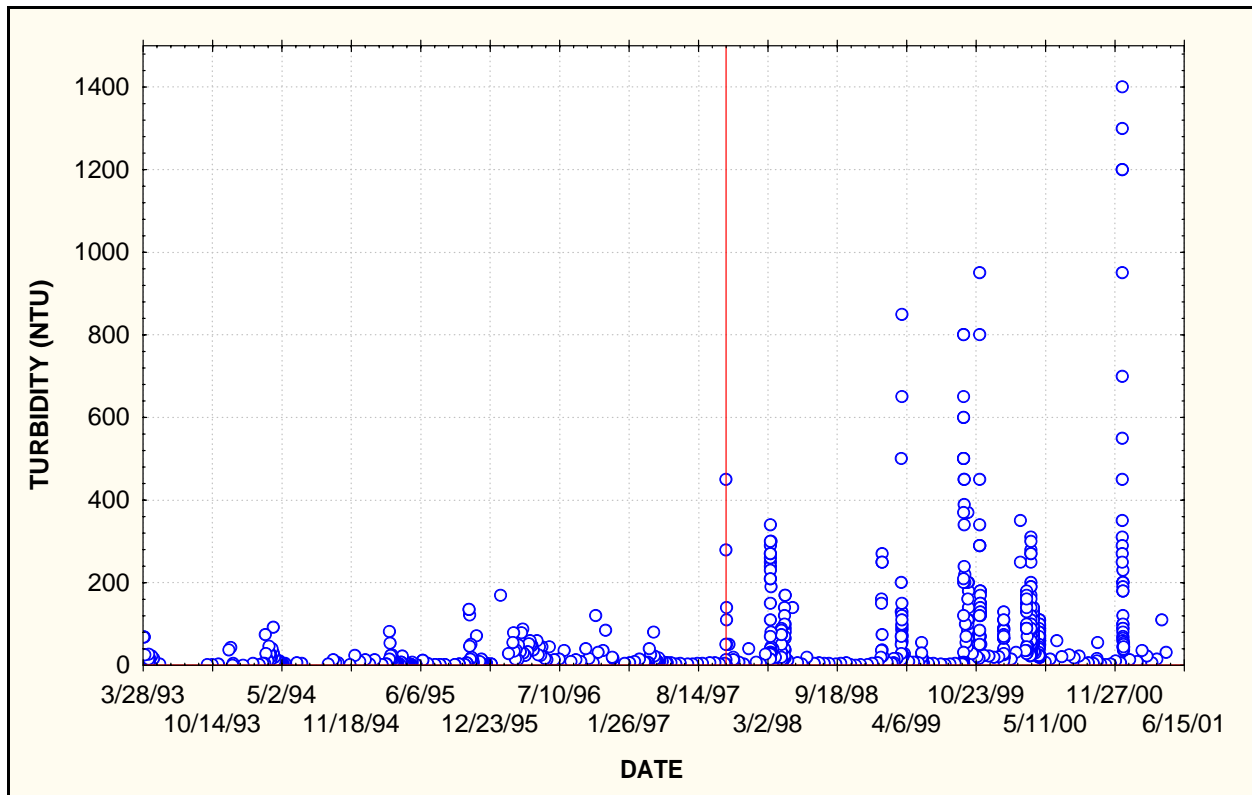
Figure V-2: Historical turbidity data for site S10 (terminal site) on the Batavia Kill.
