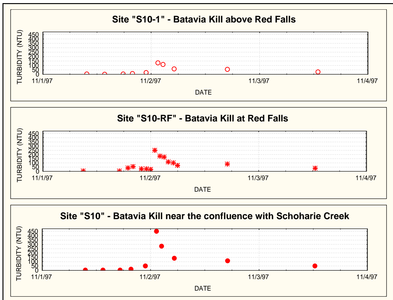
Figure V-7: Turbidity above, at , and below Red Falls November 1997.
