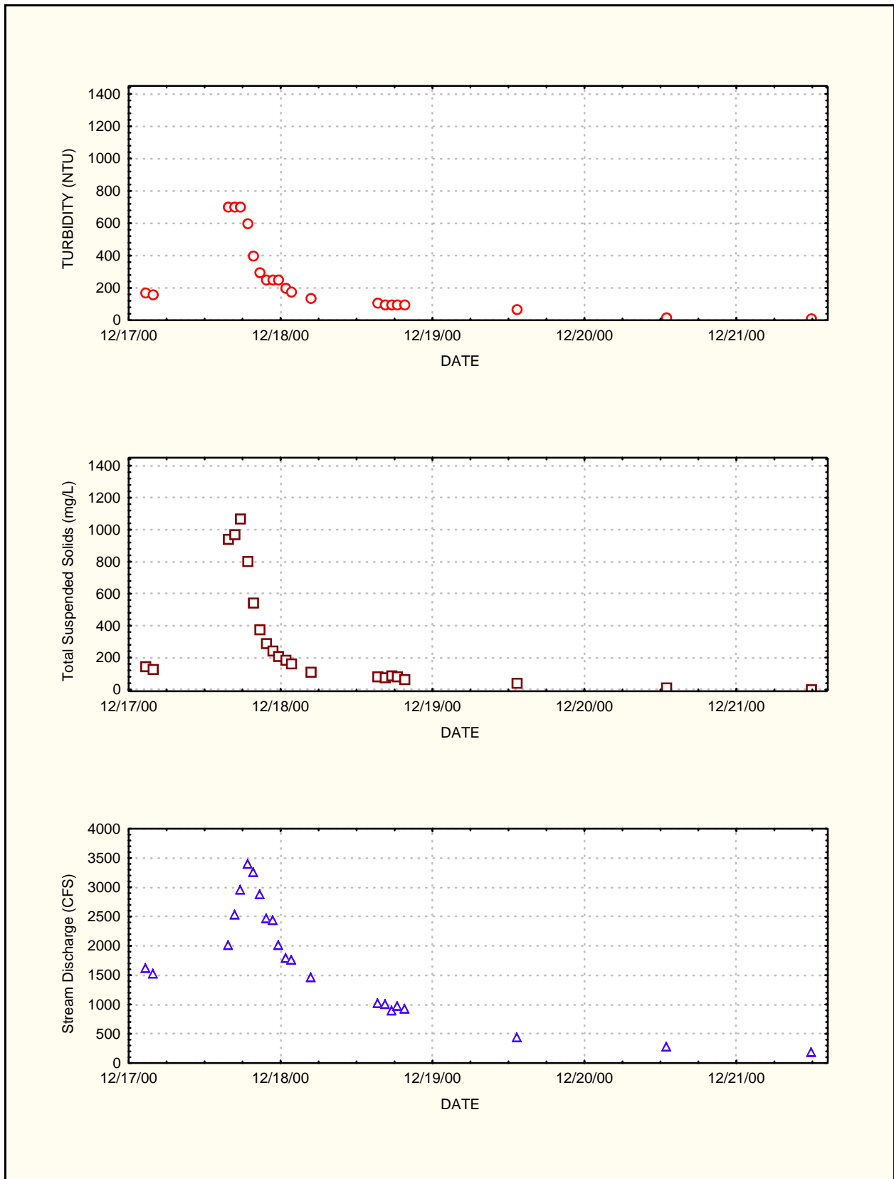
Figure V-9: Turbidity, Total Suspended Solids and Stream Discharge above Red Falls December 2000.
