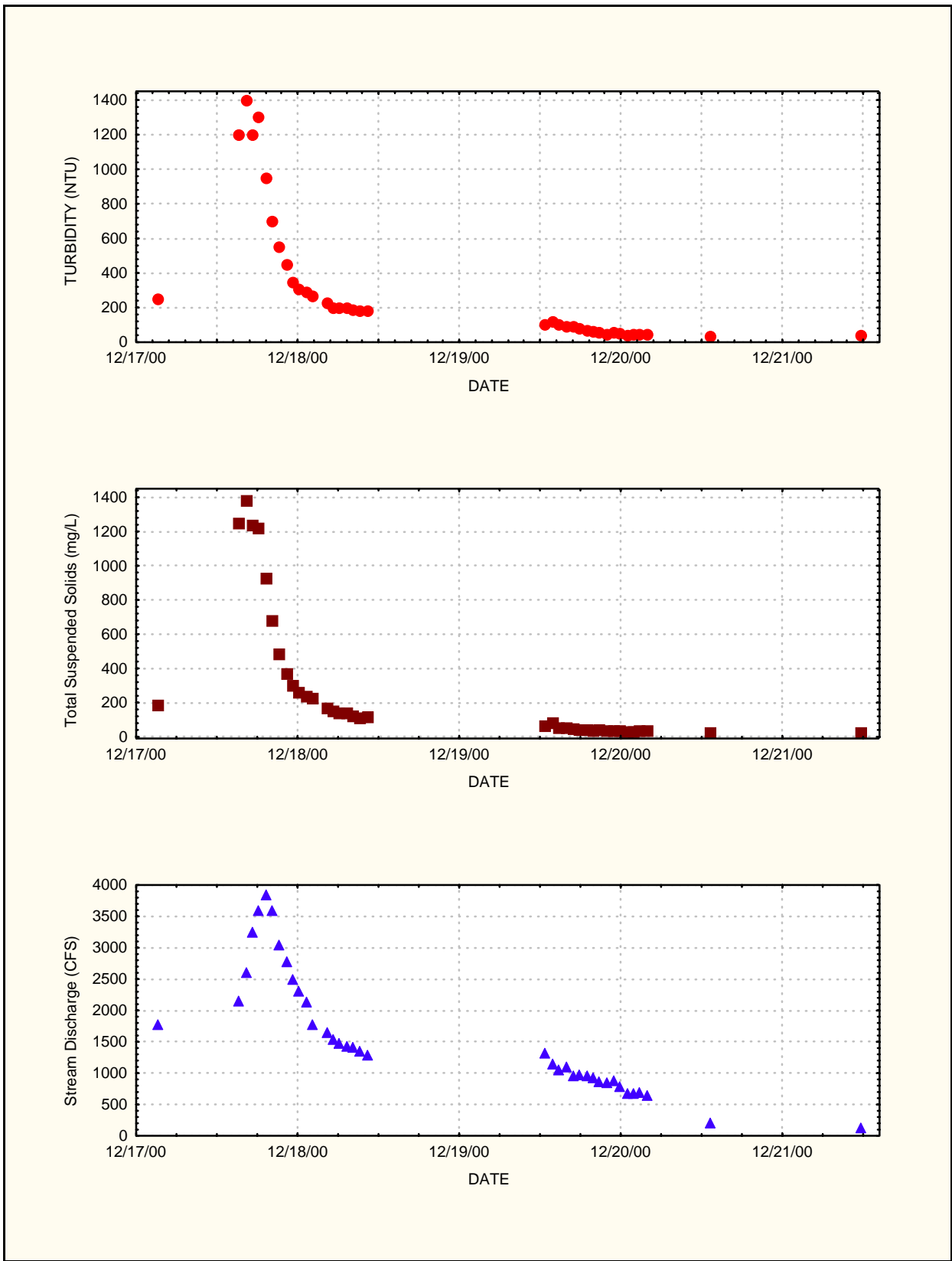
Figure V-10: Turbidity, Total Suspended Solids, and Stream Discharge below Red Falls December 2000.
