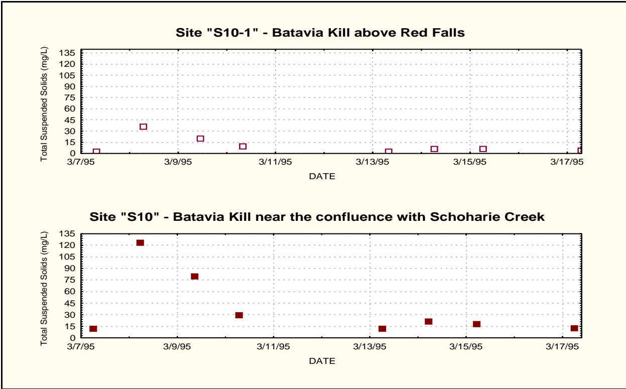
Figure V-6: Total Suspended Solids above and below Red Falls, March 1995.
